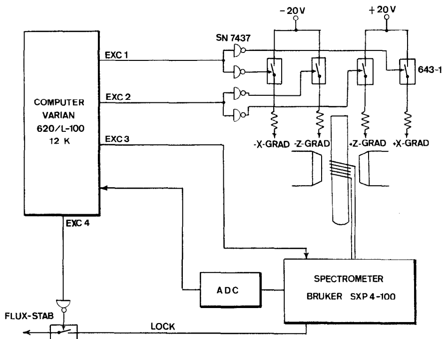
FIG. 2. Block diagram of the experimental set-up.
