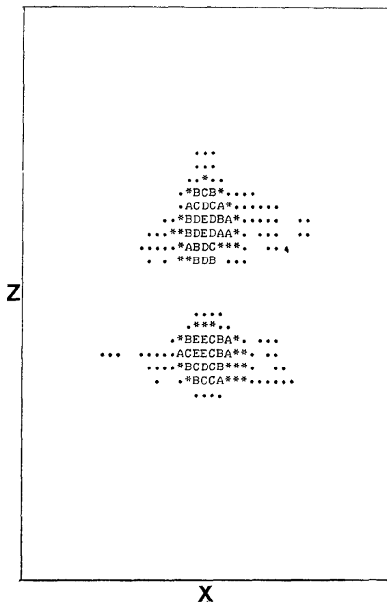
FIG. 4. The Fourier zeugmatogram obtained from the data partially shown in Fig. 3. The absolute value |\bar{\rho}(r')| of the spin density function is plotted as a function of x and z . Only the central section of the 64 \times 64 zeugmatogram is shown.
